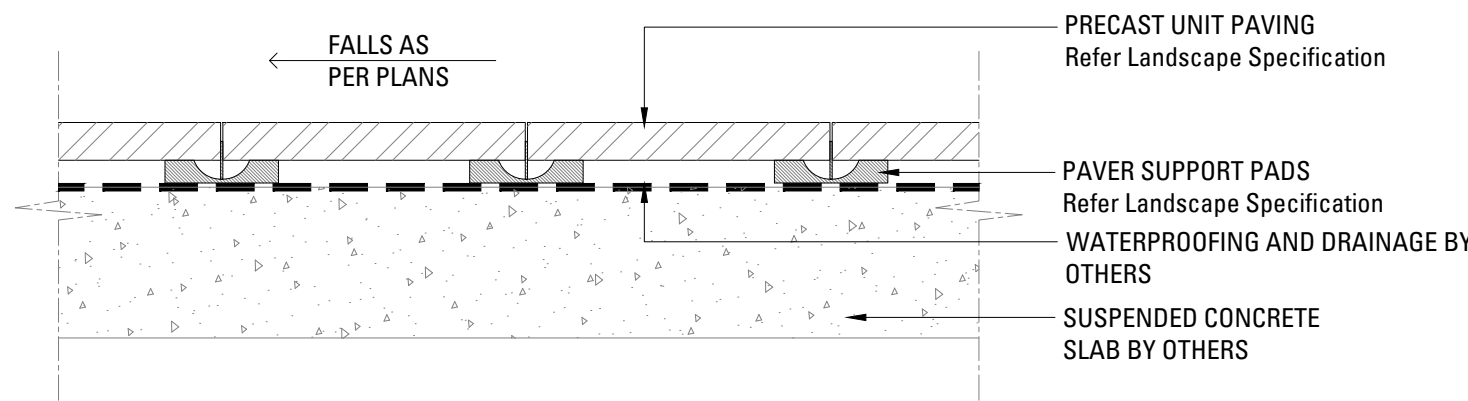
03 PRECAST UNIT PAVERS ON PADS ON SUSPENDED SLAB SCALE 1:10
