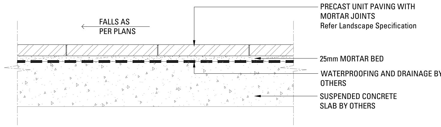
02 PRECAST UNIT PAVERS ON SUSPENDED SLAB SCALE 1:10
