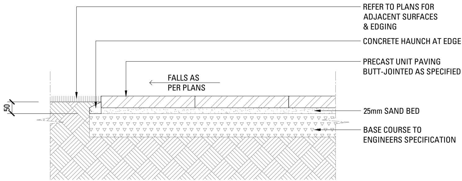
01 PRECAST UNIT PAVERS ON GRADE SCALE 1:10
