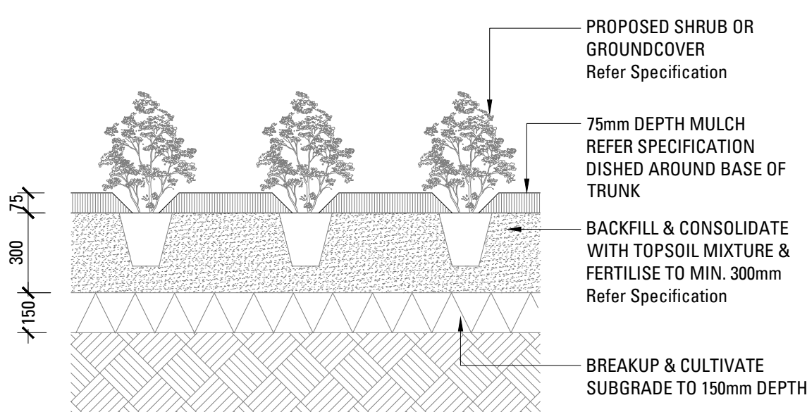
06 SHRUB OR GROUNDCOVER IN PLANTING BED SCALE 1:20
