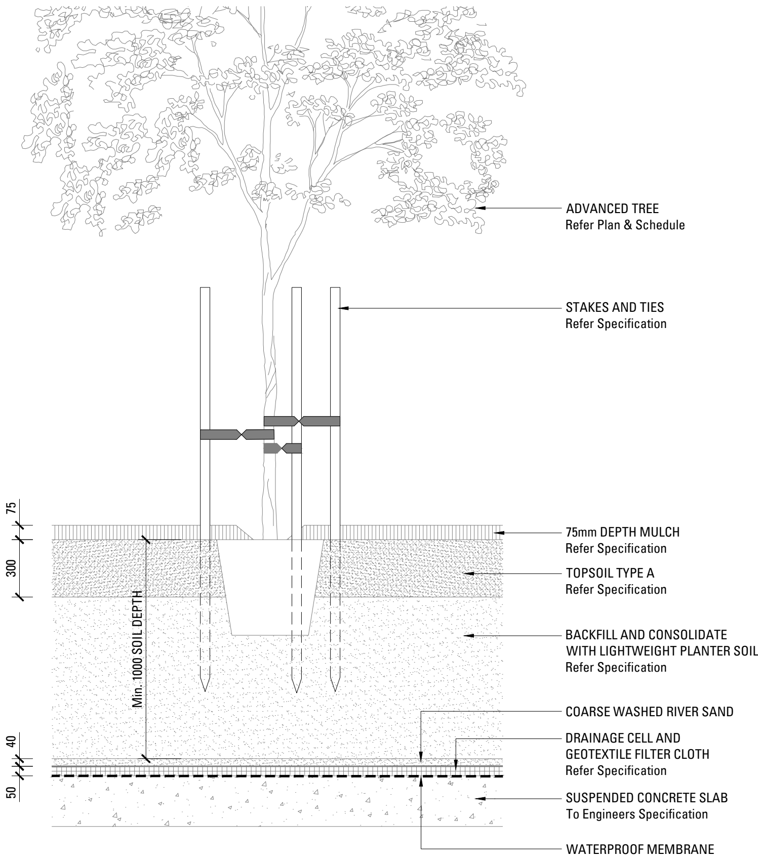
05 TREE PLANTING ON SLAB 75-100L SCALE 1:20
